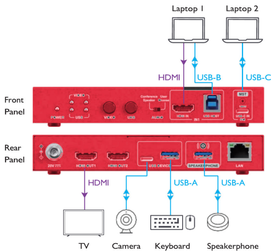
RAV-SW-2x2HU-MST diagram
