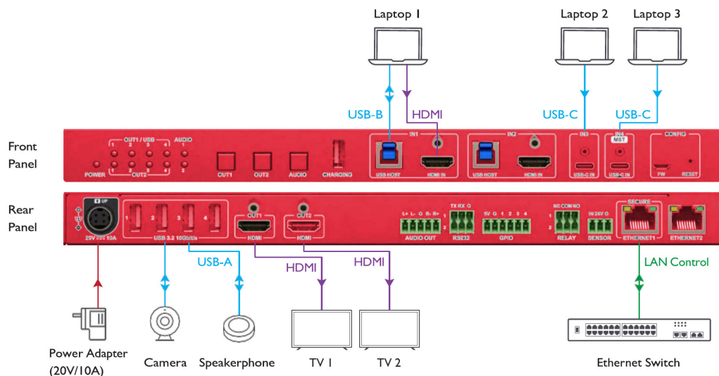
RAV-MS-4x2HU diagram
