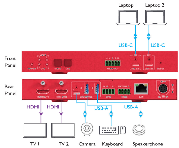
RAV-SW-2x2CU-MST-E diagram
